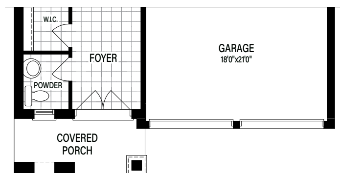
Partial Main Floor Elevation C
