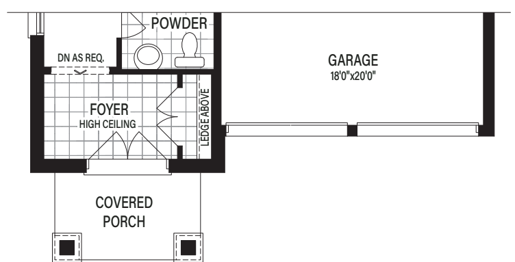
Partial Main Floor Elevation C
