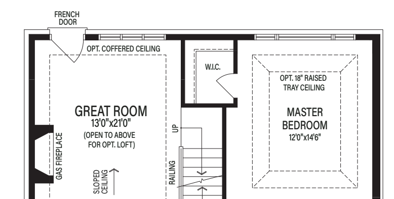
Partial Main Floor for Optional Loft Elevation A (B & C Similar)
