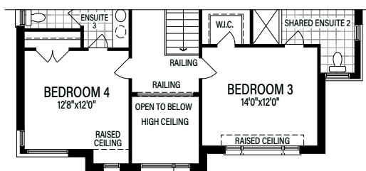
Partial Optional Second Floor Elevation C
