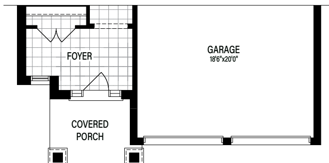
Partial Main Floor Elevation C
