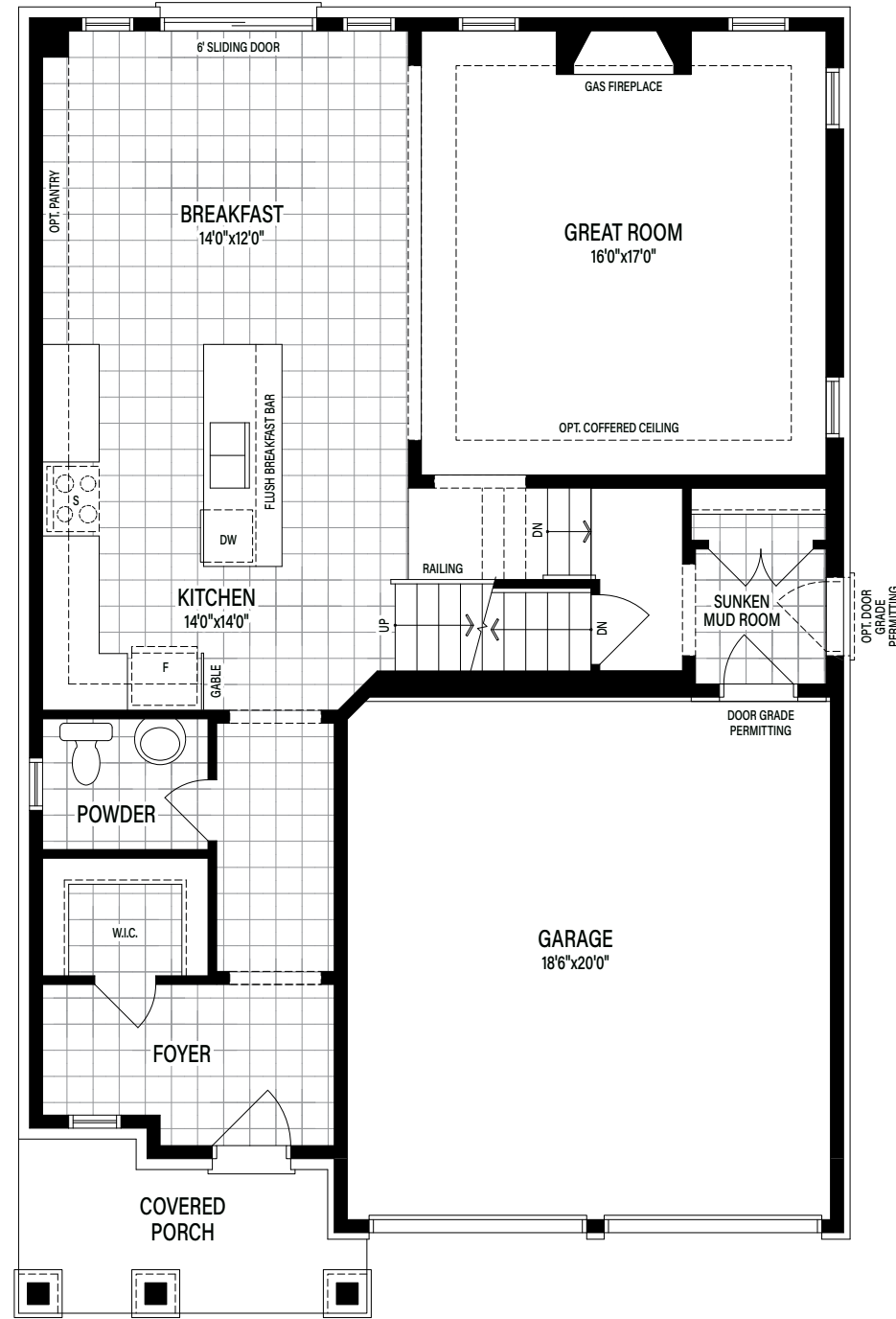
Main Floor Elevation A
