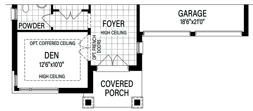
Partial Main Floor Elevation C
