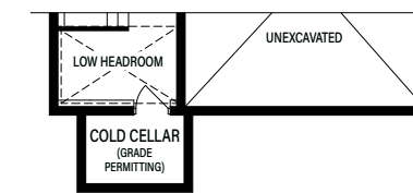
Partial Basement Elevation C
