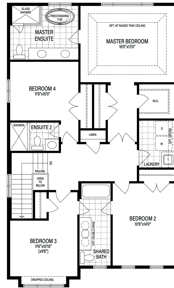
Optional Second Floor Elevation A
