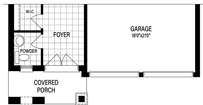
Partial Main Floor Elevation C
