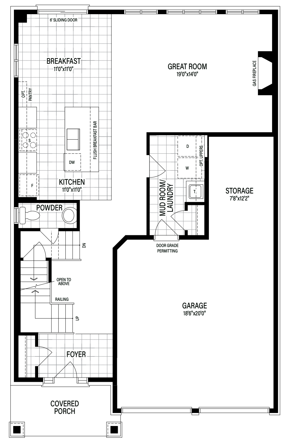
Main Floor Elevation A
