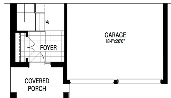
Partial Main Floor Elevation B
