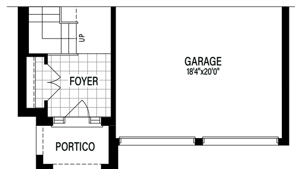
Partial Main Floor Elevation C
