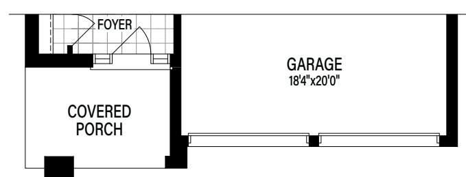
Partial Main Floor Elevation C
