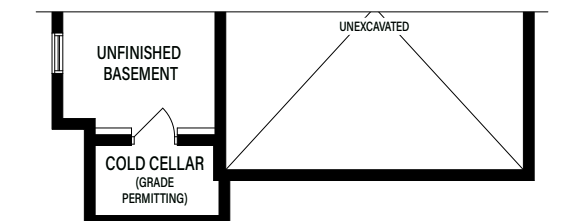
Partial Basement Elevation C
