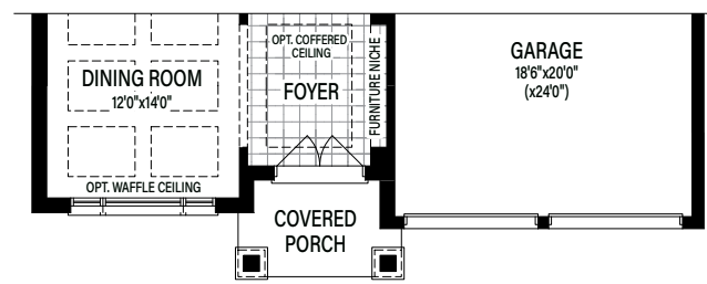
Partial Main Floor Elevation C
