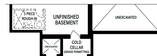
Partial Basement Elevation C
