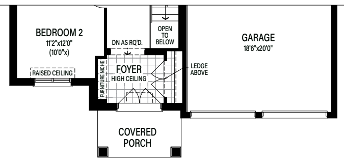
Partial Main Floor Elevation B
