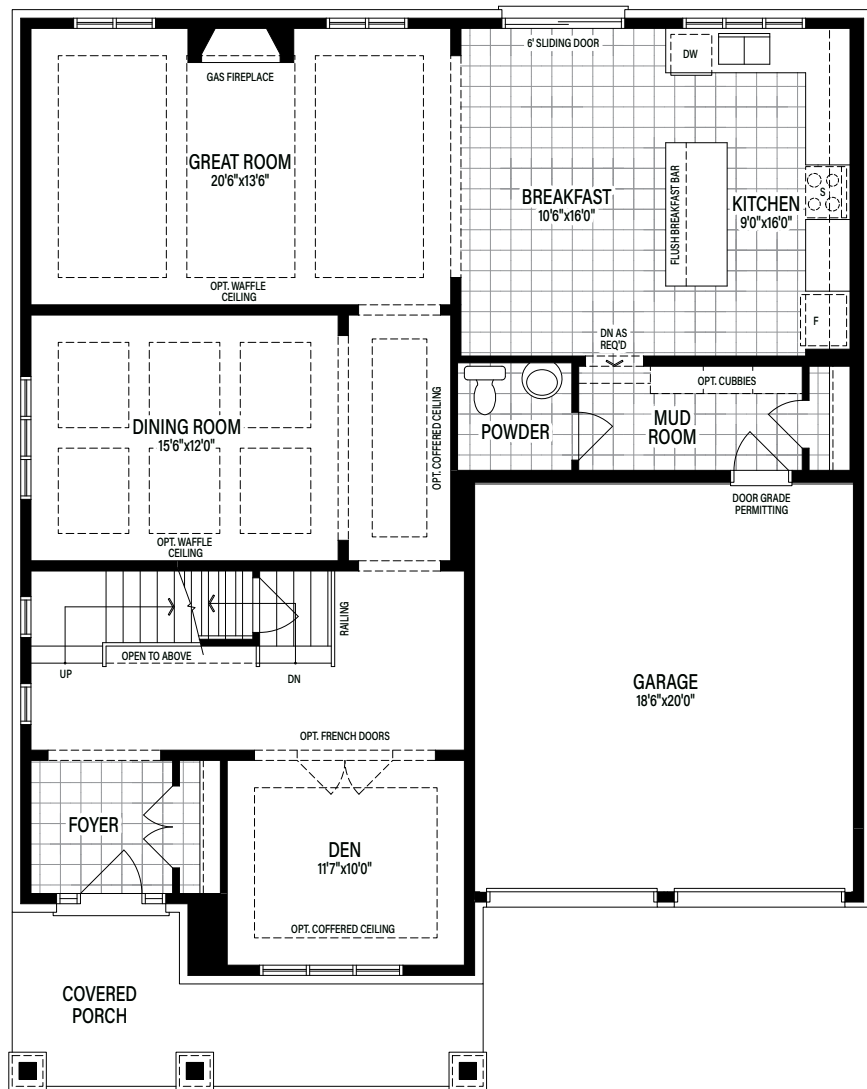
Main Floor Elevation A
