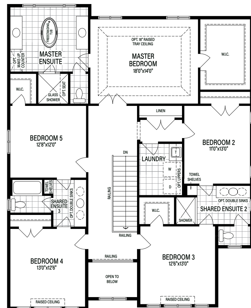
Optional Second Floor Elevation A
