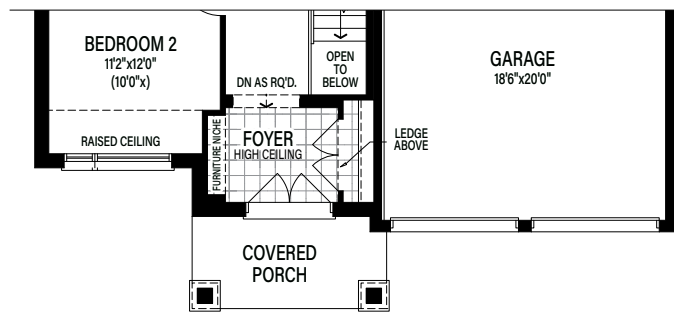
Partial Main Floor Elevation C
