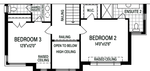
Partial Second Floor Elevation C
