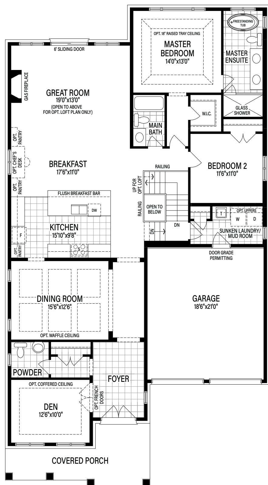
Main Floor Elevation A
