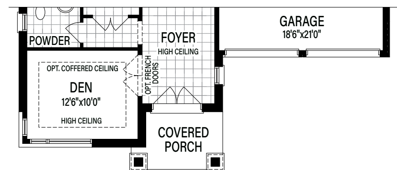
Partial Main Floor Elevation C
