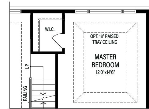
Partial Main Floor for Optional Loft Elevation A (B & C Similar)
