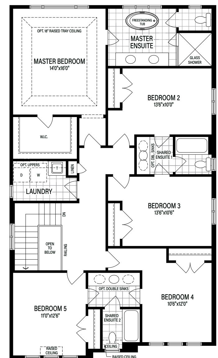
Optional Second Floor Elevation A
