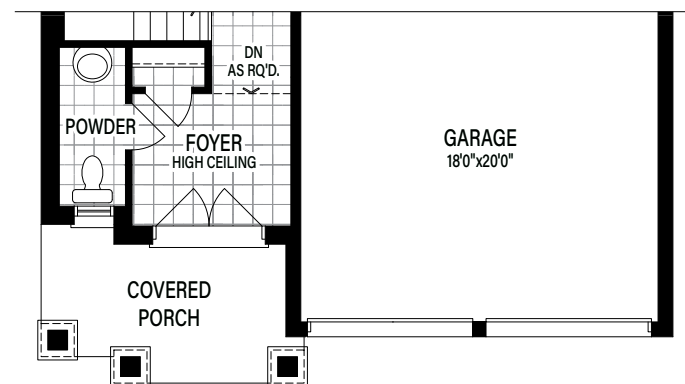
Partial Main Floor Elevation C
