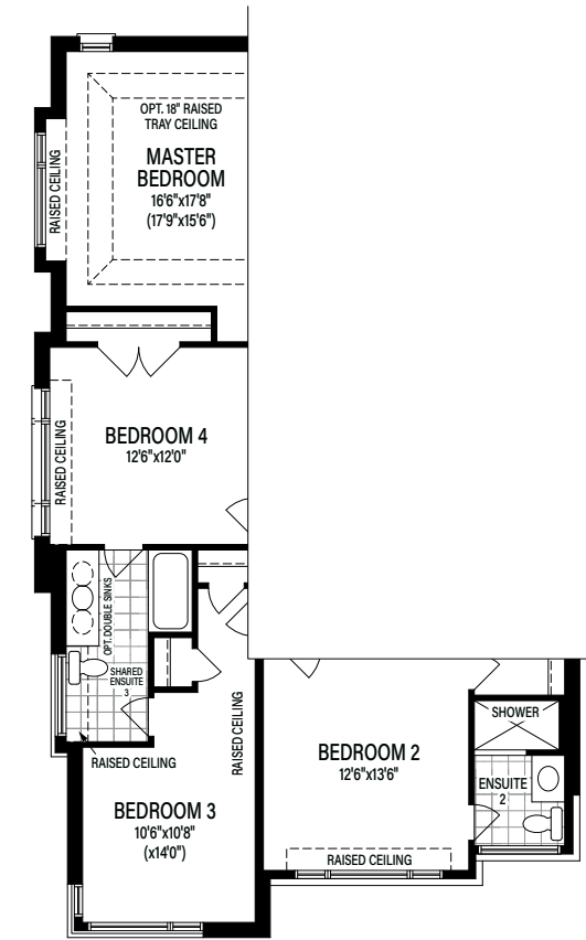
Partial Second Floor Elevation C
