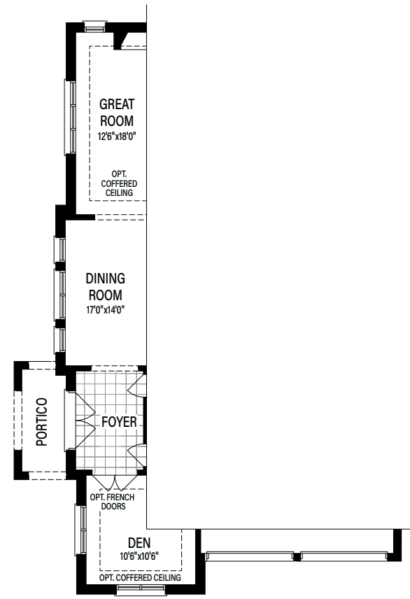
Partial Main Floor Elevation B
