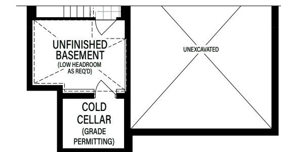
Partial Basement Elevation B
