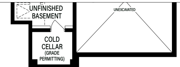
Partial Basement Elevation C
