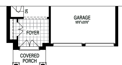
Partial Main Floor Elevation C
