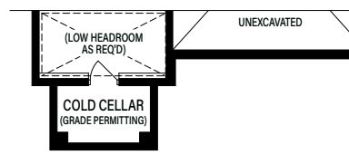
Partial Basement Elevation C
