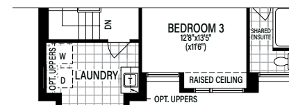
Partial Optional Second Floor Elevation C
